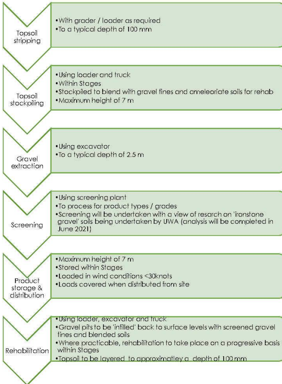
Figure 11: Gravel extraction process flow
